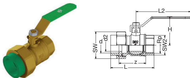
BR PP-RCT Ü-Kugelhahn-Messing IG-zyl verschraubt Runddichtring-EPDM 20°C/1,0MPa grün BR PP-RCT Transition-Ball valve Brass female-thread-cyl with union-nuts O-Ring-gasket-EPDM 20°C/1.0MPa green
