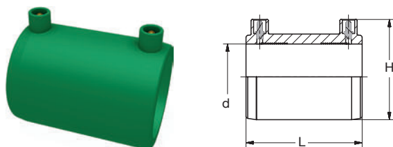
PP-RCT E-Muffe grün PP-RCT E-Socket green
