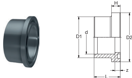
BR PVC-U Bundbuchse O-Ring-Kammer grau
