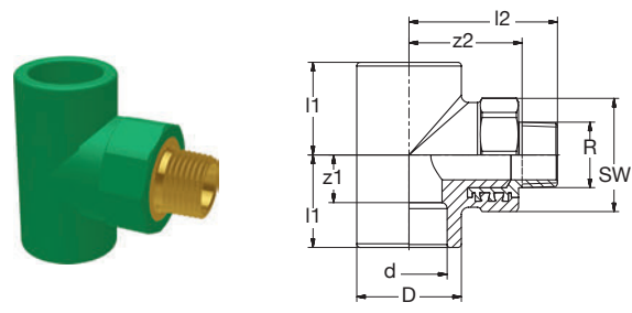
BR PP-RCT-RG/LFB Ü-T-Stück 90° AG-keg grün BR PP-RCT-Bronze/LFB Transition-Tee 90° male-thread-con green
