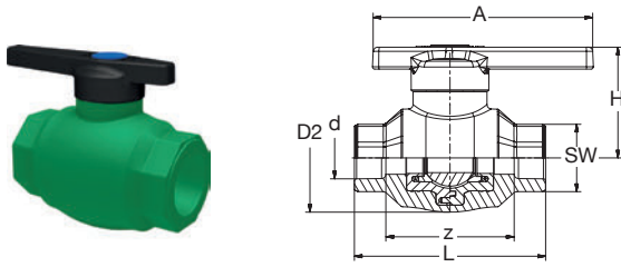
BR PP-RCT Kugelhahn 20°C/1,0MPa grün BR PP-RCT Ball valve 20°C/1.0MPa green
