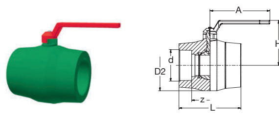
BR PP-RCT Kugelhahn 20°C/1,0MPa grün NEU BR PP-RCT Ball valve 20°C/1.0MPa green NEW
